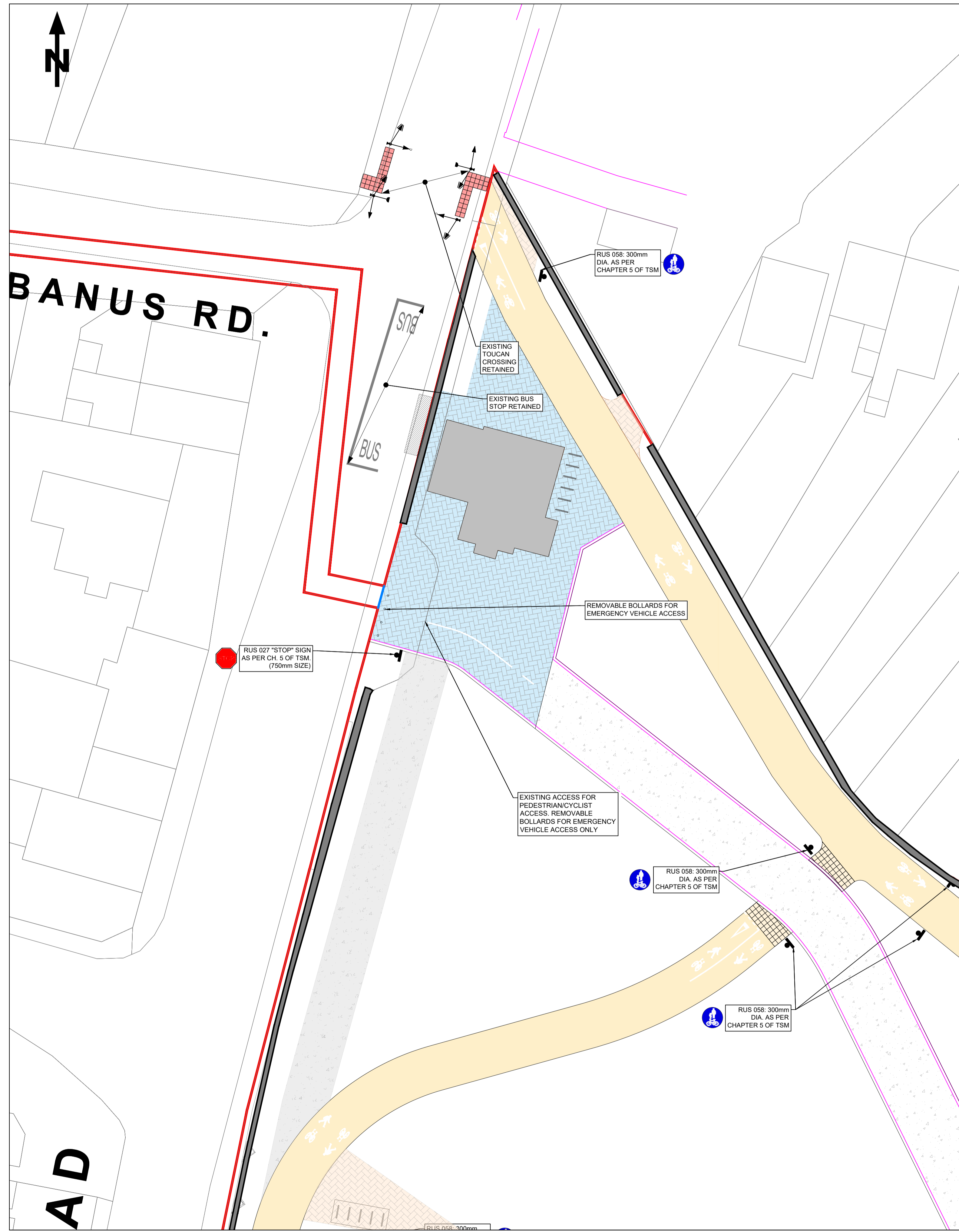
DUNDRUM ROAD ACCESS JUNCTION (SOUTH)
